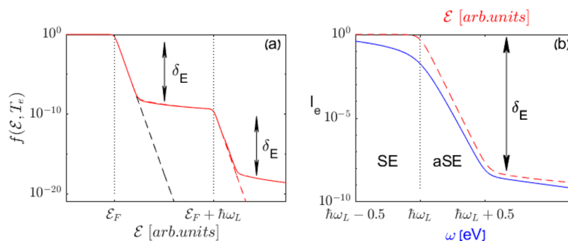
Figure 1. (Color online) (a) A typical nonequilibrium electron distribution f(\epsilon) (3). Here, |\hat{E}_L|^2 = 5 \times 10^{10} [\text{V}^2/\text{m}^2] , \hbar\omega_L = 2.25 \text{ eV} , and \epsilon_{Ag} = -8.5 + 1.8i . The theoretical prediction for the “hot” electron distribution (3) (red dashed line) is in excellent agreement with the full numerical result (red solid line). The thermal distribution at the steady-state electron temperature is shown by the dashed black line. (b) The electronic contribution to the emission (6) (blue solid line) compared to the distribution f(3) (dashed red line).
